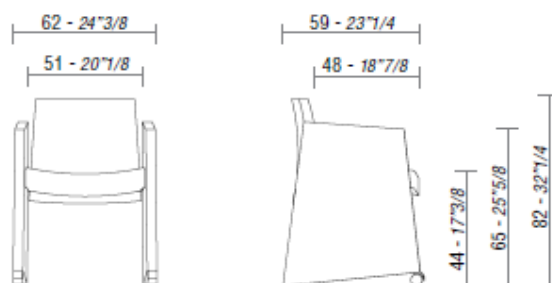
M2, single seat tub chair.
